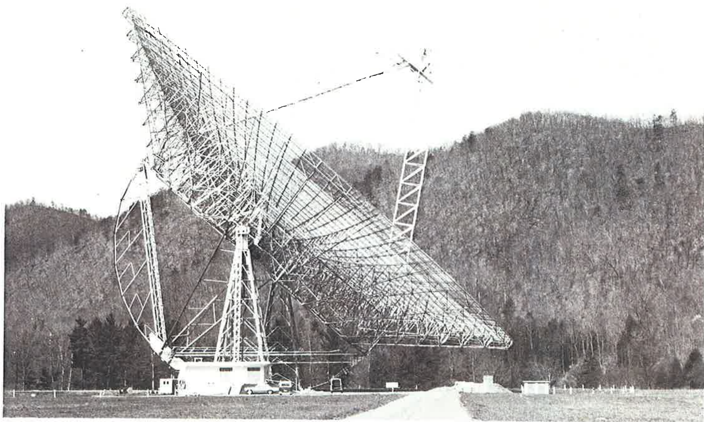
Survey telescope. The 91-meter transit radio telescope at the National Radio Astronomy Observatory in Green Bank, West Virginia
